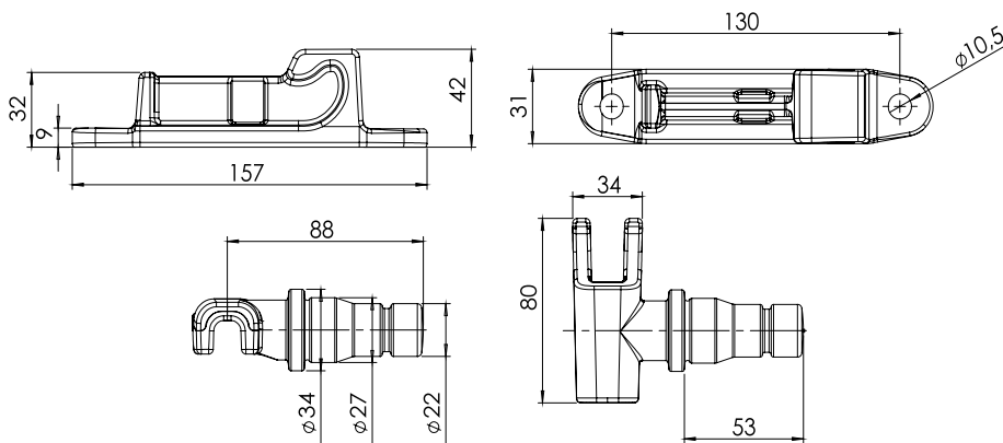
CAM AND KEEPER Ø27
